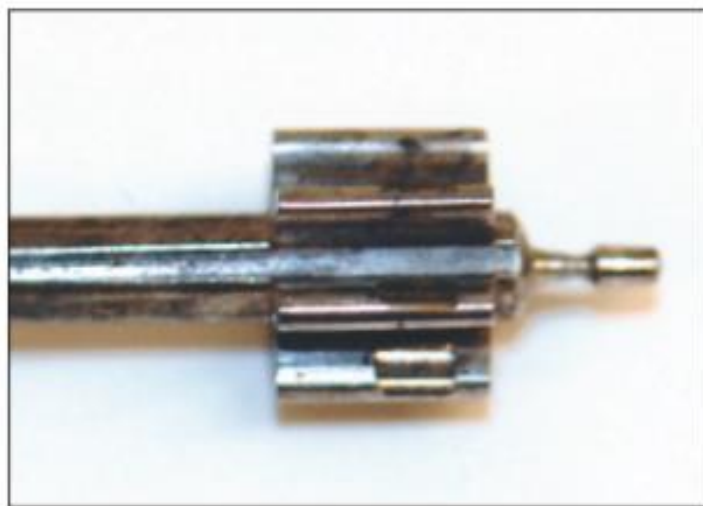
Figure 22. The damaged pivot is cut off.
