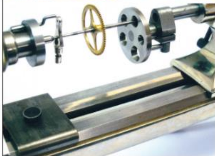
Figures 19A and 19B. The cone plate supporting the centre arbor at the pinion leaves.
