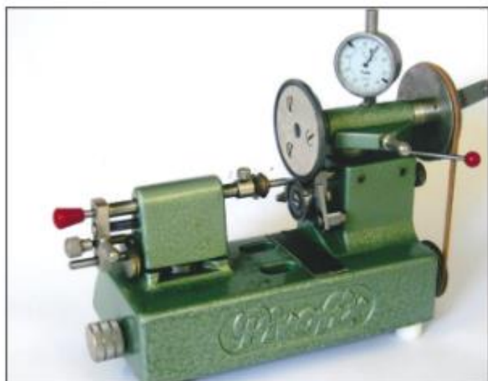
Figures 12 and 13. A burnishing tool by Bergeon.
