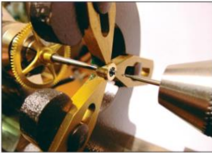
Figure 24. The arbor is held in the collet.
