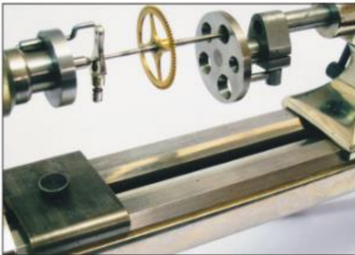
Figure 26. The work being supported between centres.
