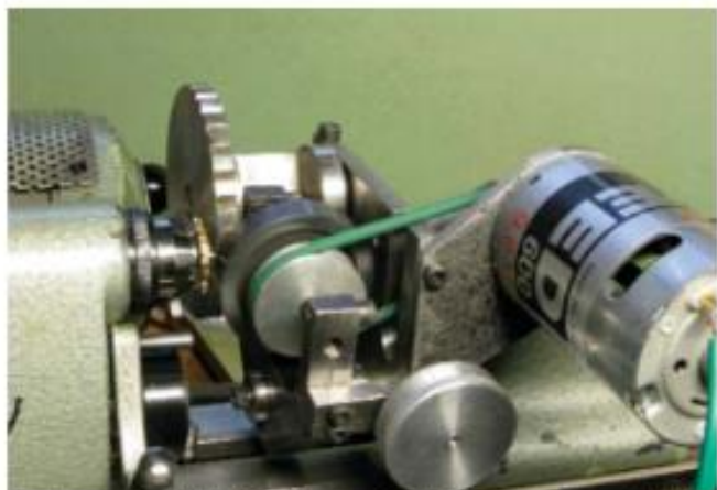
1. A pocket watch balance having the bottom pivot burnished in a Boley F1 watchmakers lathe.
