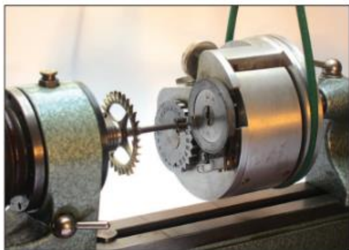
Figure 14. The Rollimat pivot polisher.
